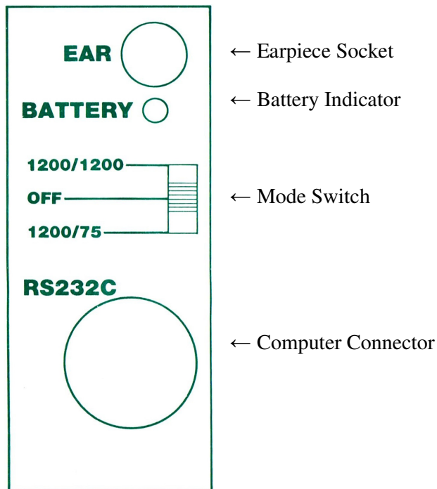
Fig. 1 Front Panel.
